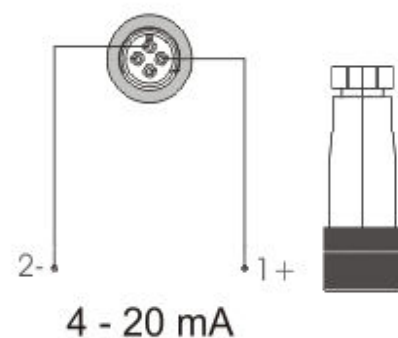
Connection schematics :
